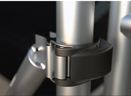
EASY-LOCK COUPLERS OPTION ON STABILISERS
