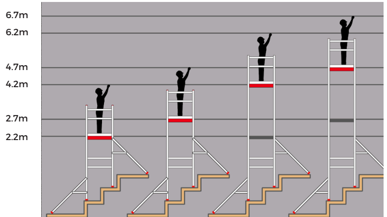
MiSTAIRS 4.2m MiSTAIRS 4.7m MiSTAIRS 6.2m MiSTAIRS 6.7m
